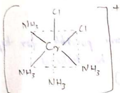
cis form
