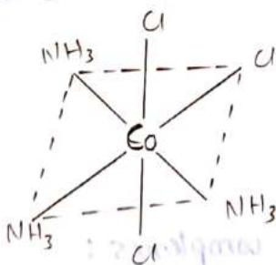
trans form
