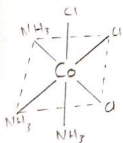
cis form
