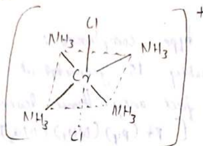
trans form
